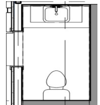
FLOORPLAN
