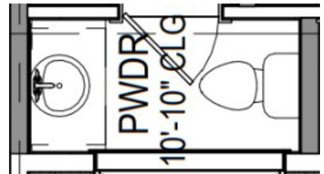
FLOORPLAN
